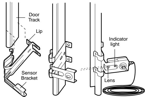
Figure 2 DOOR TRACK MOUNT (Right Side)
