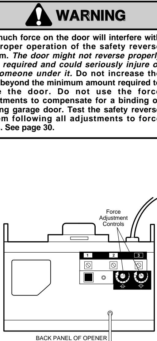
BACK PANEL OF OPENER
